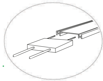
Insert the copper pin of the module in the track under the copper bar
